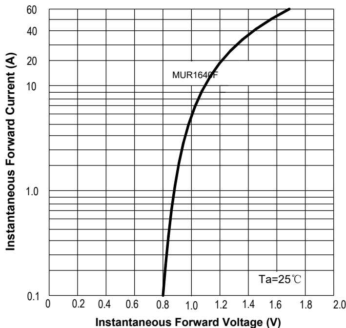
FIG3: Forward Voltage
