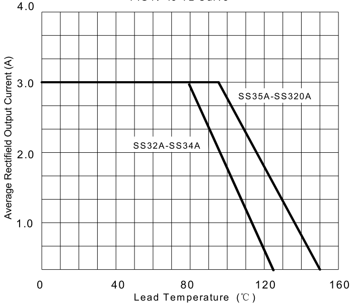
FIG1: Io-TL Curve
