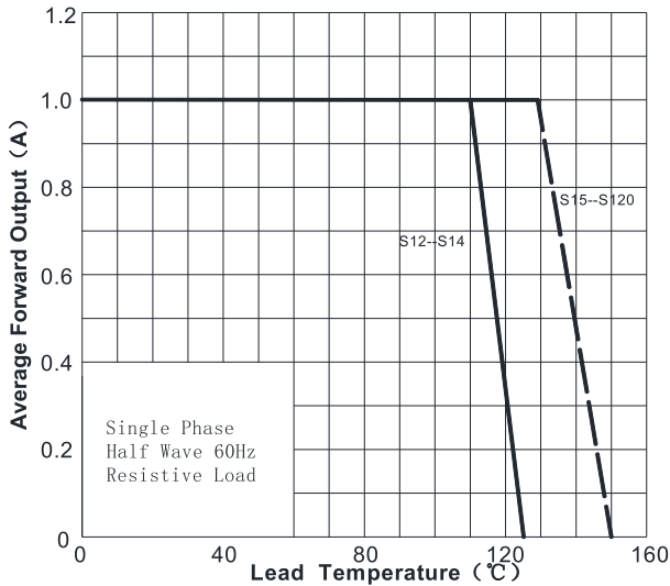
FIG1:Io-TL Curve
