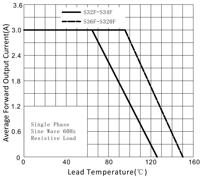
FIG1:Io-TL Curve
