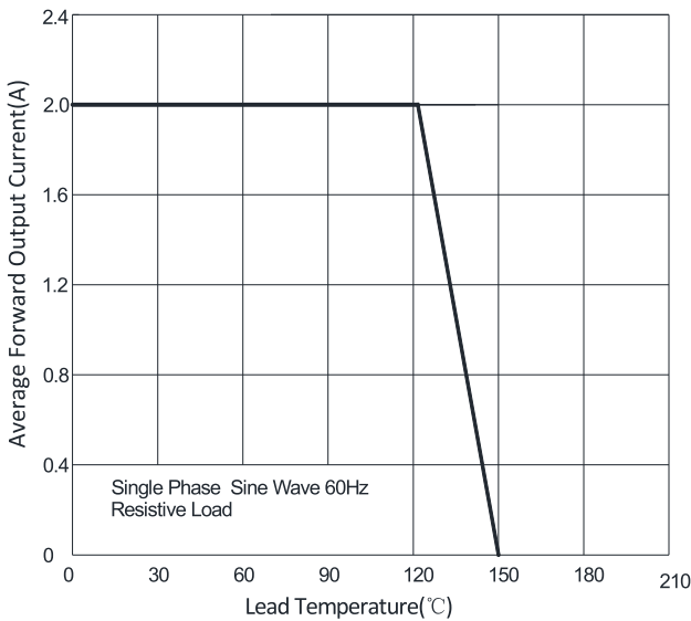
FIG1: Io-TL Curve
