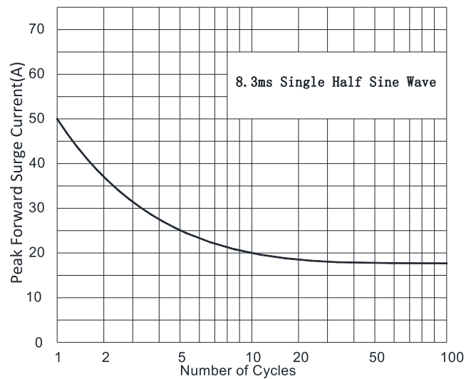
FIG2: Surge Forward Current Capadity
