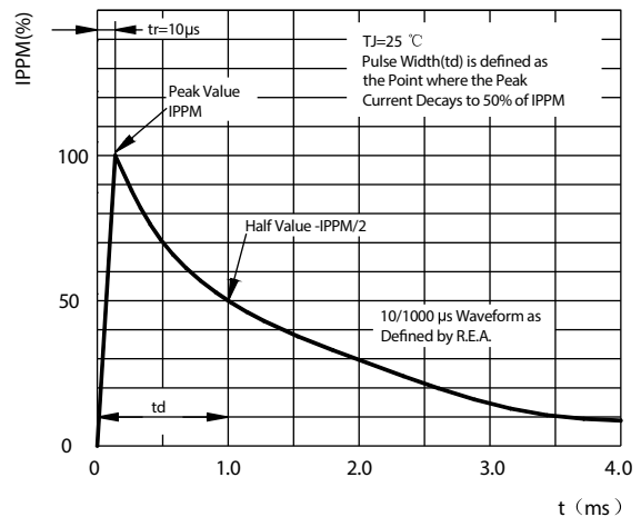
FIG2: Pulse Waveform
