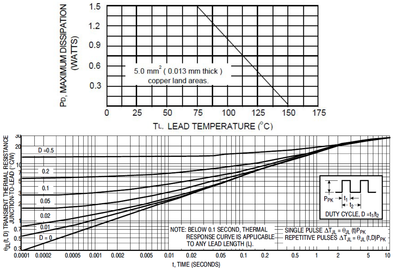
Figure 2. Typical Thermal Response L, Lead Length = 3/8 Inch
