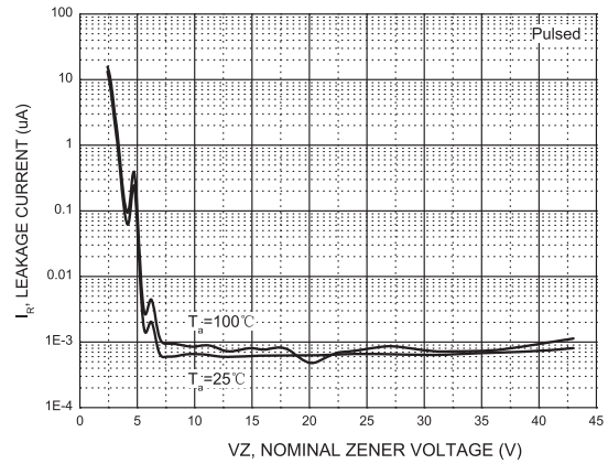
FIG.4-Typical Leakage Current
