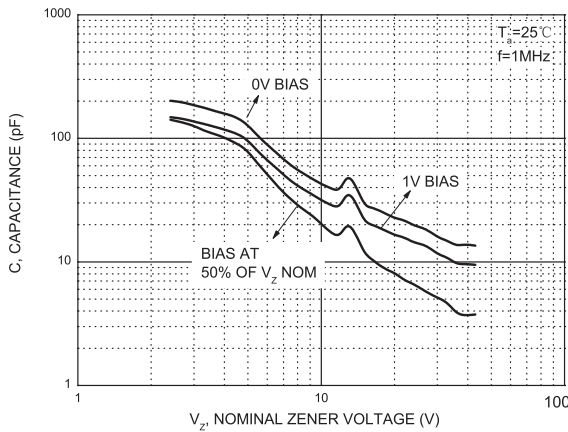
FIG.5-Typical C Capacitance
