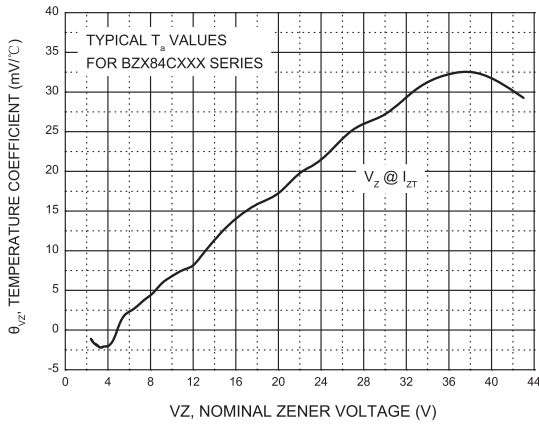
FIG.3- Temperature Coefficients
