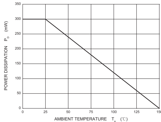
FIG.7-Power Derating Curve
