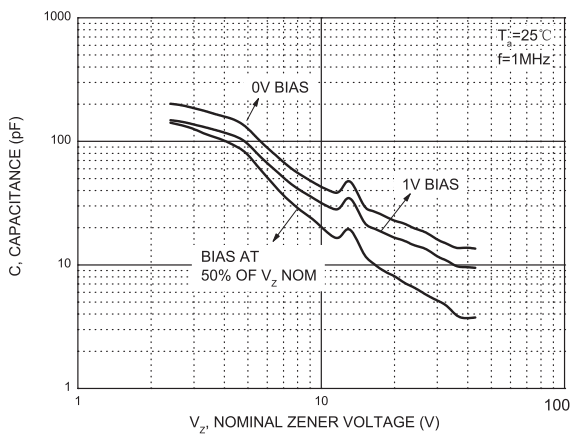
FIG.5-Typical C Capacitance
