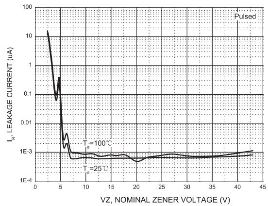
FIG.4-Typical Leakage Current
