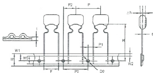
Fig. 1 Epoxy Coated F=5 and 7.5mm (RT1 or RT2)
