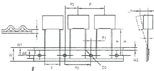
Fig. 2 Box F=5 and 7.5mm (RT1 or RT2)
