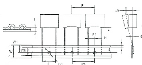
Fig. 3 Box Fitch=7.5mm Ammo Only (RT2)
