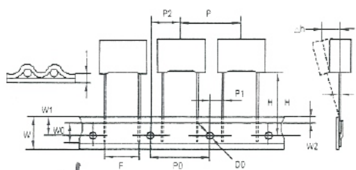
Fig. 4 Box or Epoxy Coated F=10 - Ammo Only F=15 Every other space skipped because of Larger body - Ammo Only (RT3 or RT4)
