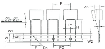
Fig. 3 Box Fitch=7.5mm Ammo Only (RT2)
