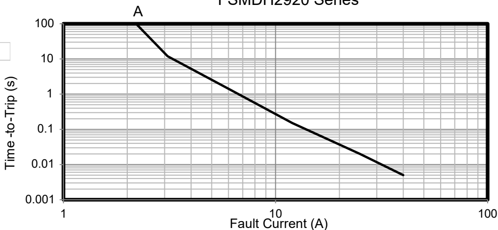
FSMDH2920 Series
