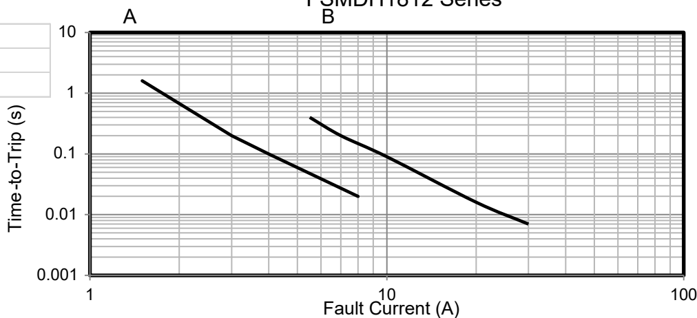
FSMDH1812 Series
