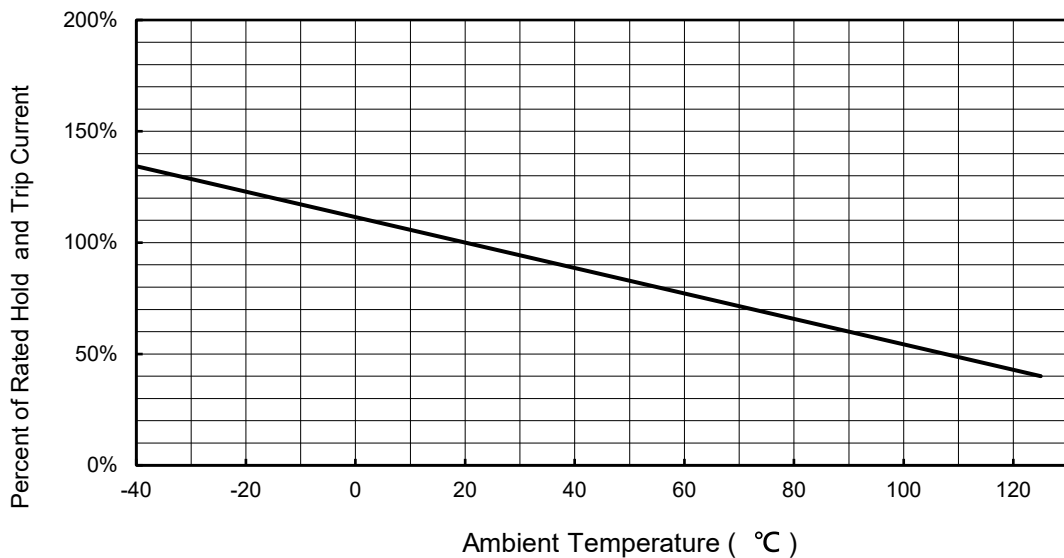
FSMDH Series
