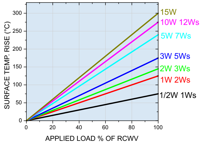
HOT-SPOT TEMPERATURE
