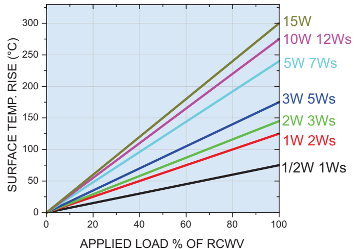
HOT-SPOT TEMPERATURE
