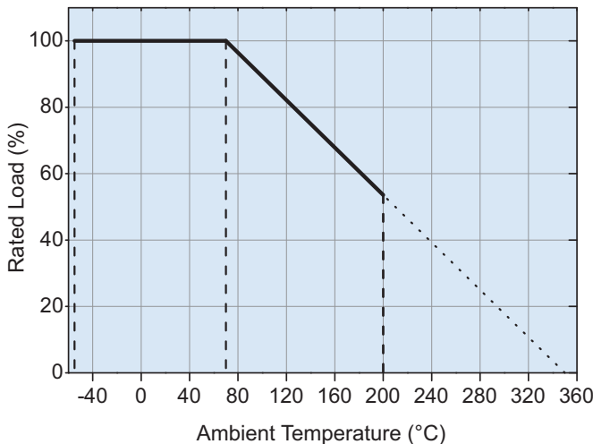
DERATING CURVE
