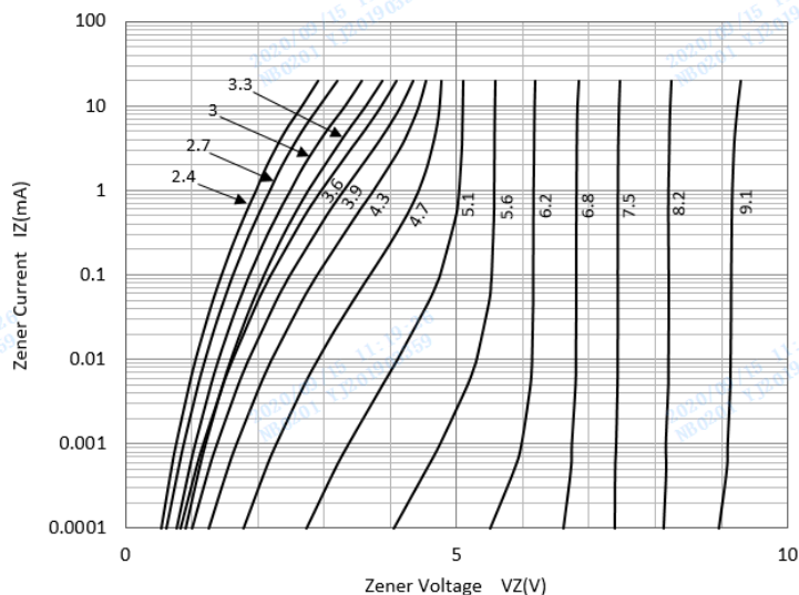
Zener Breakdown Characteristics
