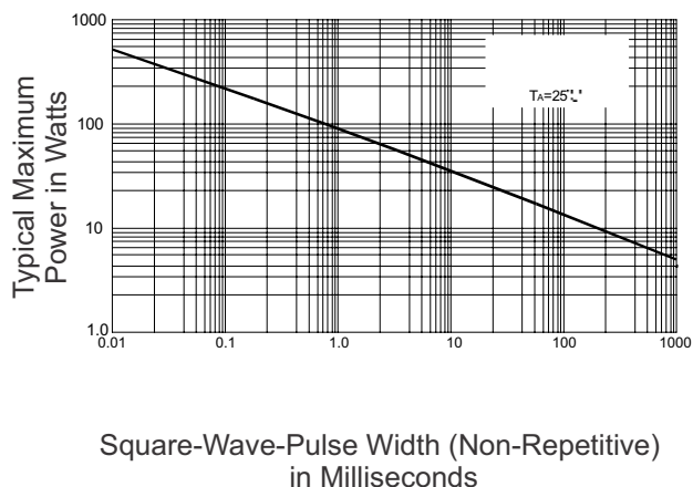
Fig. 2 - Transient Surge Capability
