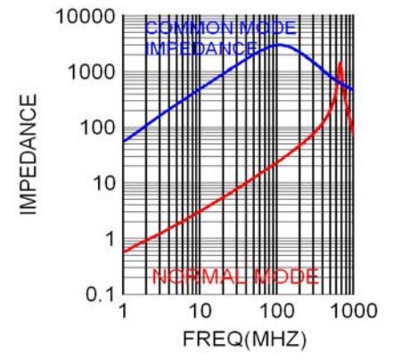
WCM-4532AUTO-272A10T
