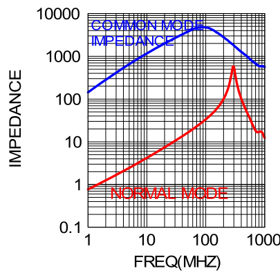
WCM-3225AUTO-220YT
