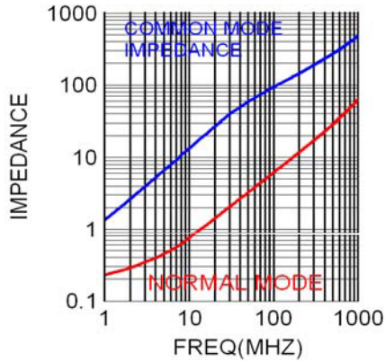
WCM-2012AUTO-900T01
