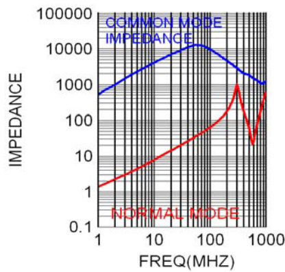
WCM-3225AUTOG-B00YT01
