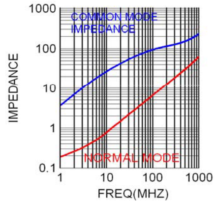
WCM-2012HSAUTO-900T
