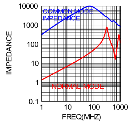
WCM-3225AUTO-510YT
