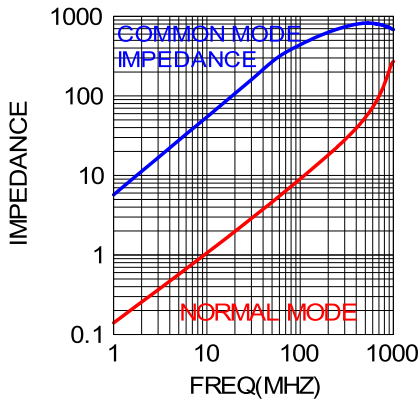
WCM-4532AUTO-421A32T13
