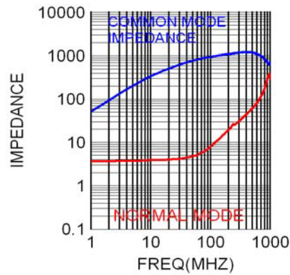
WCM-4532AUTO-102A21T
