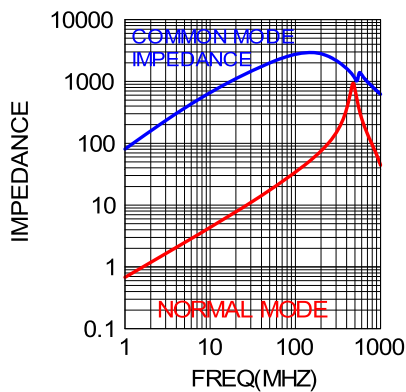
WCM-3225AUTO-110YT
