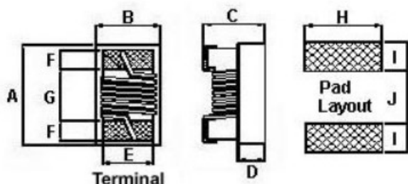
SCS0402
