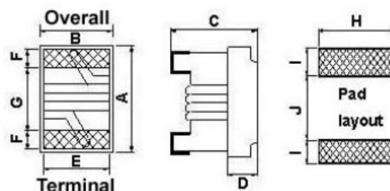
SCS0603/0805/1008
